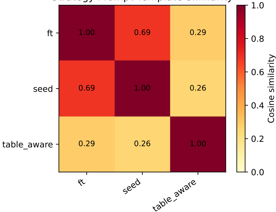
Strategy Prompt Template Similarity
